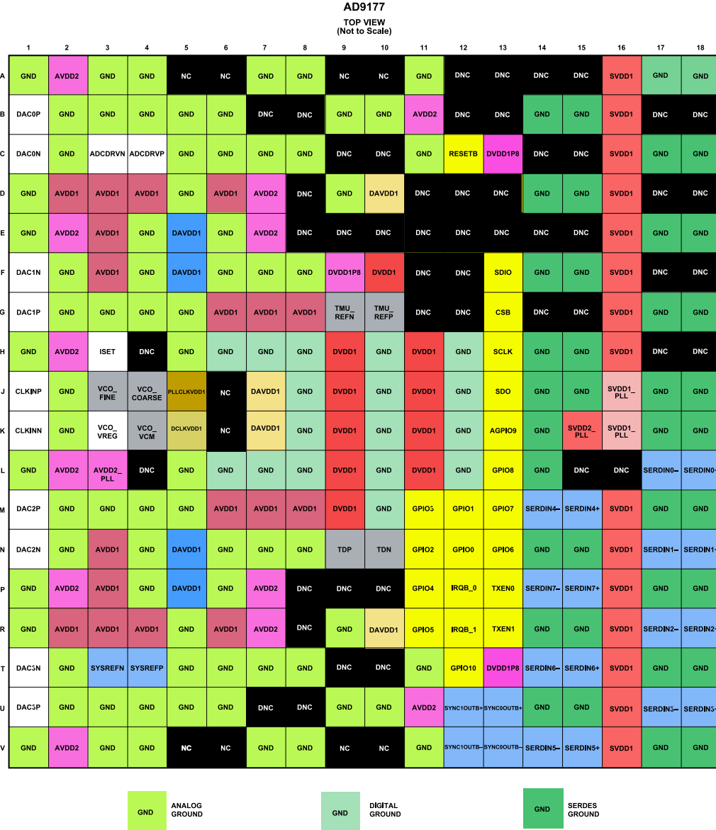
Figure 5. Pin Configuration
