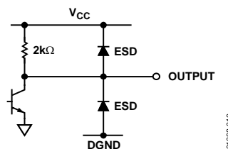
Figure 47. Logic Output
