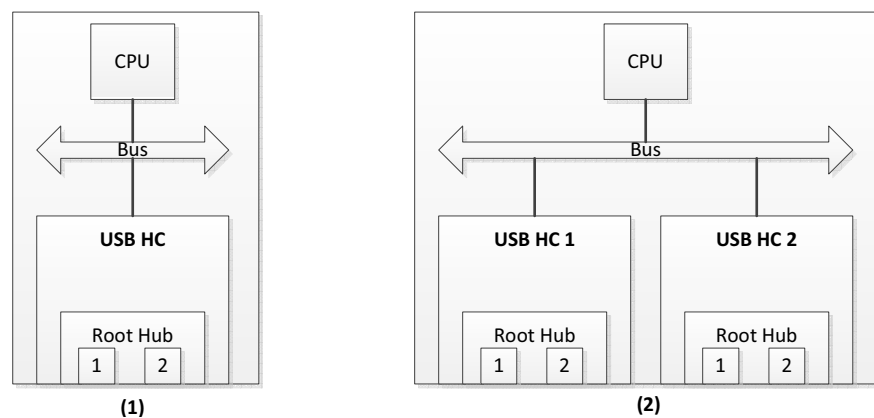
Figure 4-2 Typical Host Controller Architectures
