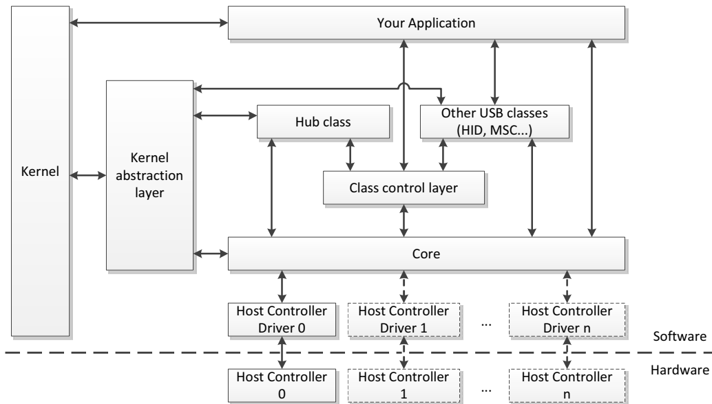
Figure 9-1 \mu\text{C}/\text{USB} -Host Interactions with the Kernel
