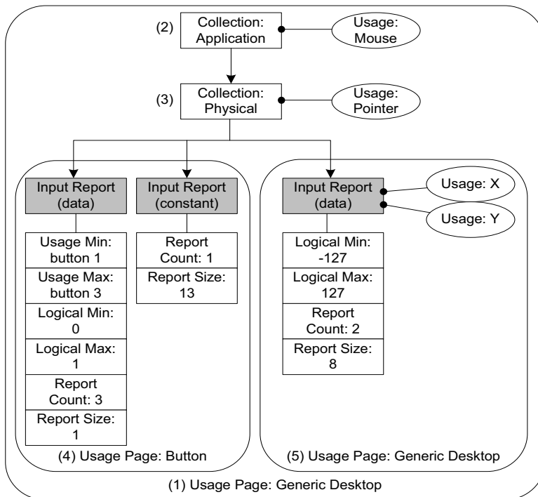
Figure 7-1 Report Descriptor Content from a Host HID Parser View
