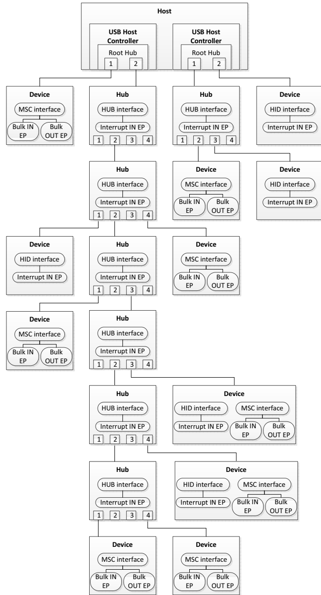
Figure 4-6 Multi-Host Controllers and Multiple Devices Configuration
