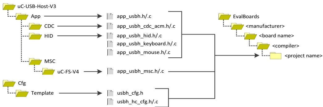
Figure 2-3 Copying Template Files.
