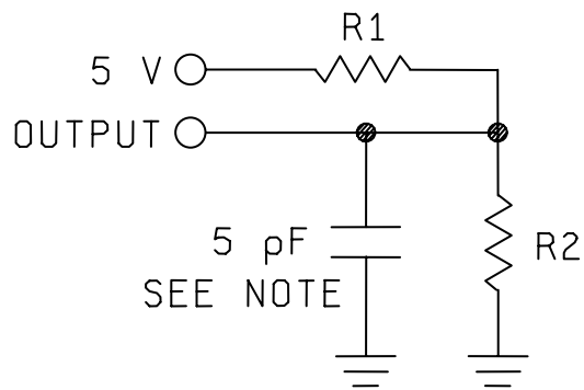
CIRCUIT B OUTPUT LOAD FOR t_{HZC} AND t_{HZE}
