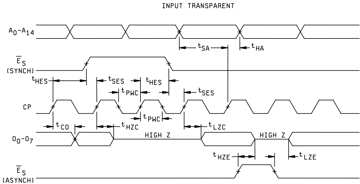
FIGURE 4. Switching waveforms.
