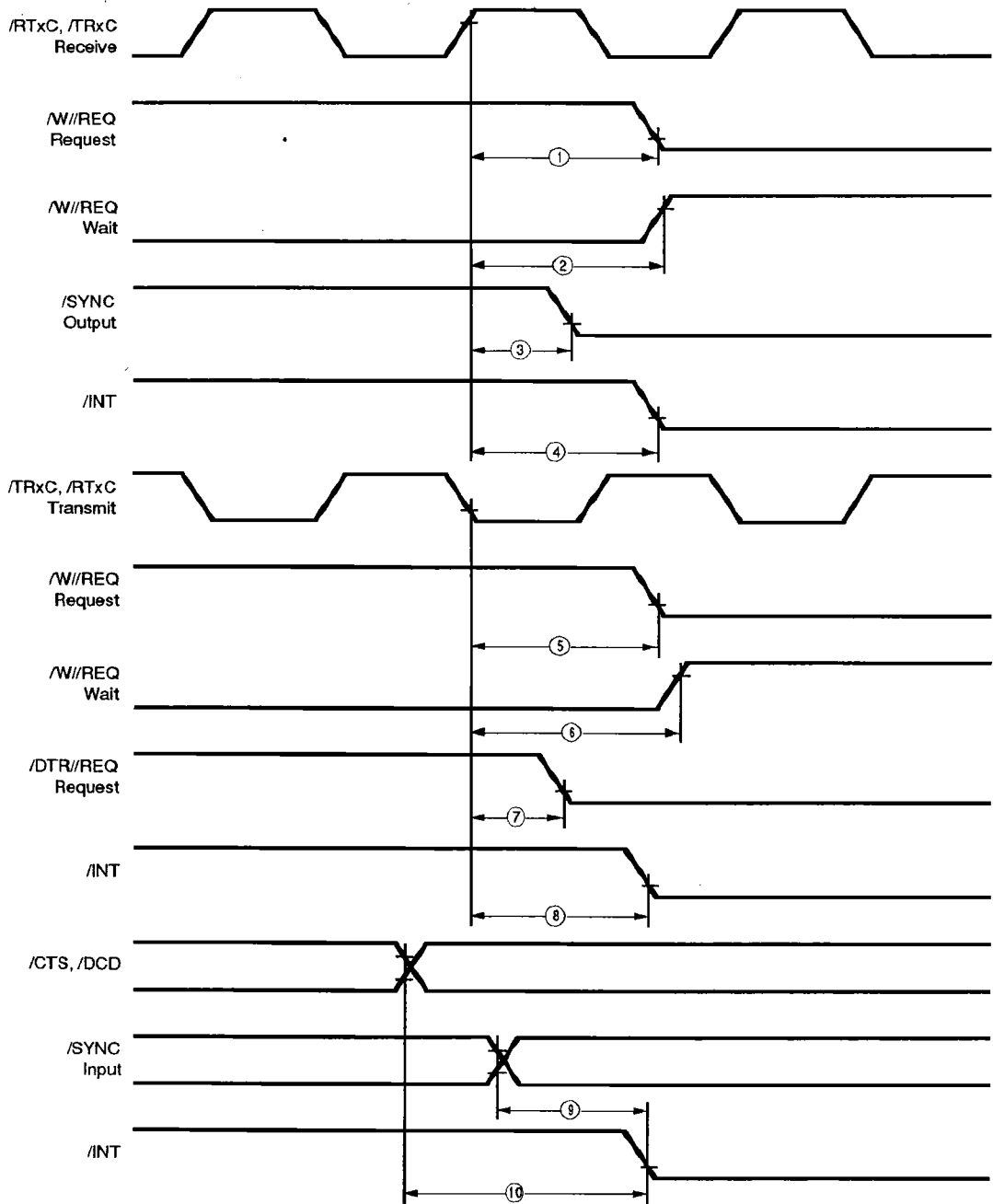
Figure 37. Z8030 System Timing Diagram
