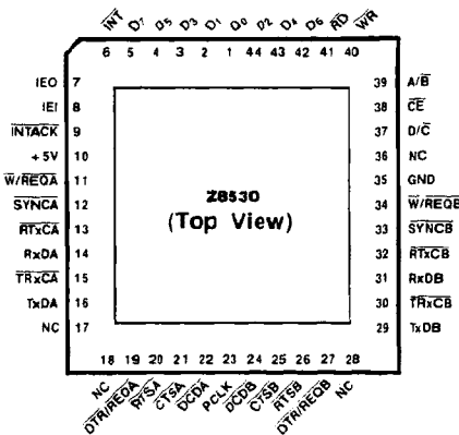
Figure 2c. Chip Carrier Pin Assignments, Z8530
